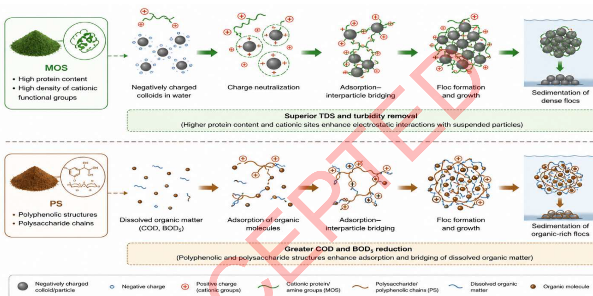
Figure 3: Coagulation–flocculation mechanism of Moringa oleifera seed (MOS) and avocado pear seed (PS) bio-coagulants. Created with BioRender.com.
