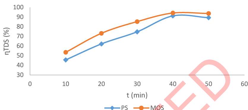
Figure 6: Effect of treatment time on TDS removal.
