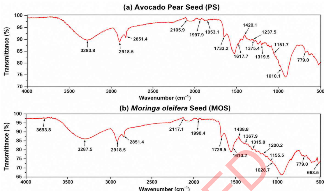
Figure 1: FTIR spectra of (a) avocado pear seed (PS) and (b) Moringa oleifera seed (MOS) bio-coagulants, illustrating the characteristic absorption peaks used for functional group identification.
