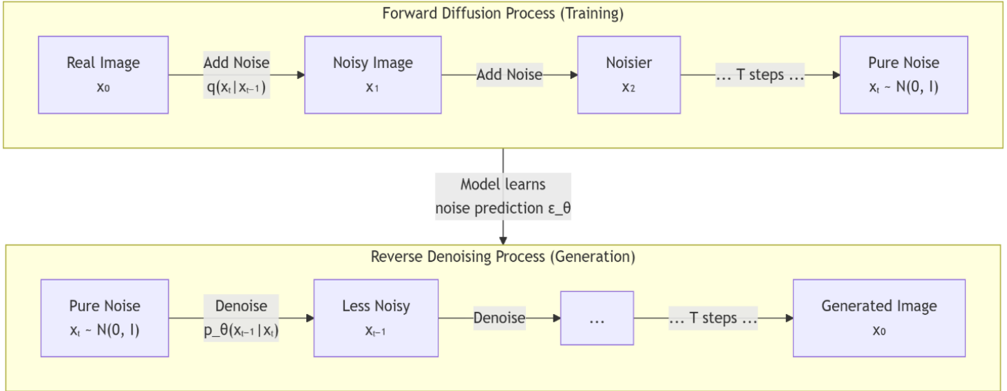
Figure 1 Schematic overview of the diffusion model pipeline. (Top) Forward diffusion: a real image is progressively corrupted by adding Gaussian noise over T steps until it becomes pure noise. The model is trained to predict the noise added at each step. (Bottom) Reverse denoising: starting from pure noise, the trained model iteratively removes predicted noise to reconstruct an image. The generation process is stochastic — different random noise seeds produce different outputs from the same learned distribution.
