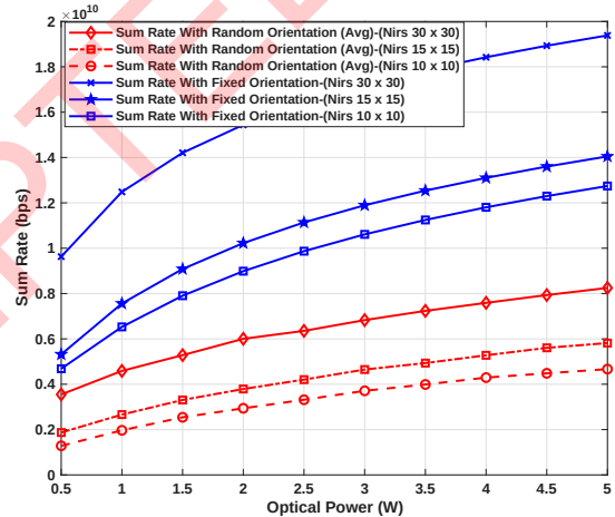
Figure 5: Sum rate comparison under fixed vs. random orientation, with time delay modeled and IRS configuration optimized via DQL.
