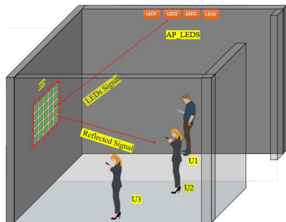
Figure 1: System model with an IRS installed on a wall.
