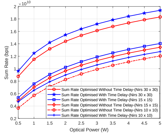
Figure 4: Impact of IRS-induced time delay on sum rate performance across different IRS sizes.
