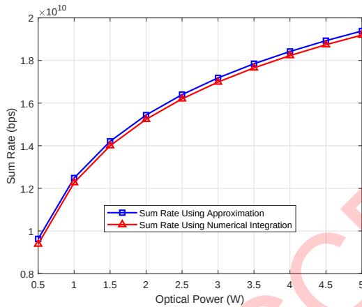
Figure 3: Validation of the derived sum rate approximation against numerical integration. Both results are computed using DQL-optimized configurations, but use different rate evaluation methods.
