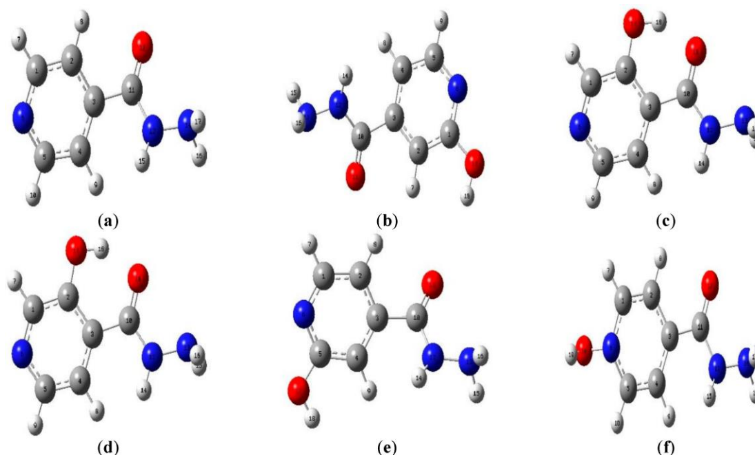
Figure 1: Optimized structures of (a) INH, (b) INH OH1, (c) INH OH2, (d) INH OH4, (e) INH OH5, and (f) INH OHN.
