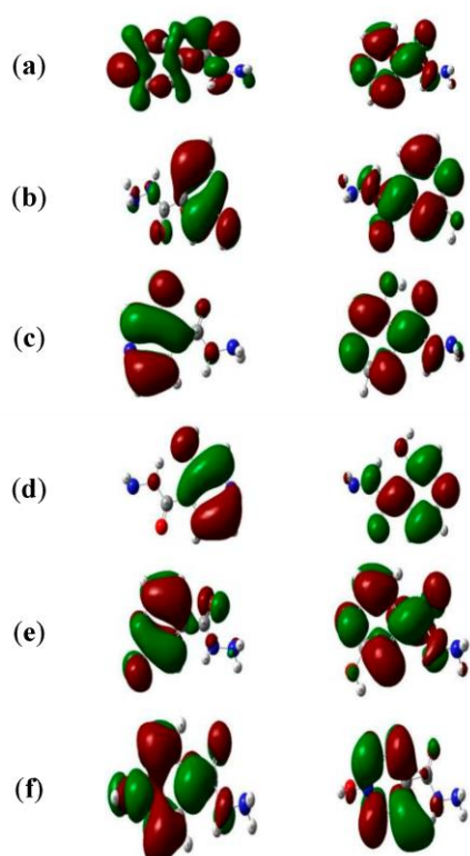
Figure 2: Orbitals involved in the electronic transition of (a) INH, (b) INH OH1, (c) INH OH2, (d) INH OH4, (e) INH OH5, and (f) INH OHN for the Highest Occupied Molecular Orbital (HOMO) and Lowest Unoccupied Molecular Orbital (LUMO), respectively.
