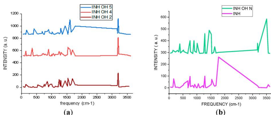
Figure 3: Simulated IR spectra of the studied INH molecule: (a) with -OH at carbon atoms 2, 4, and 5, and (b) INH molecule and INH with -OH at N atom.
