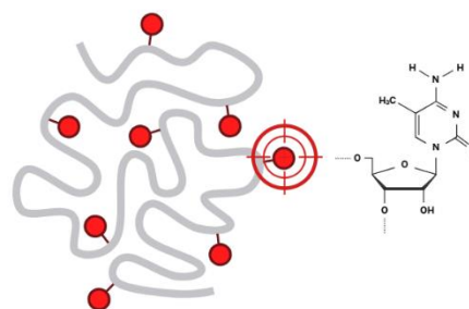
Figure 2 illustrates DNA methylation as a heritable epigenetic modification in which a methyl group ( -CH_3 ) is covalently added to the 5th carbon position of the cytosine ring, typically within cytosine-guanine (CpG) dinucleotides. The process is catalyzed by DNA methyltransferases (DNMTs), a family of enzymes that play a key role in establishing and maintaining methylation patterns. This modification is essential for regulating gene expression, preserving genomic stability, and guiding cell differentiation and development. Created with https://app.biorender.com/illustrations/683913466895553df7df7bc5
